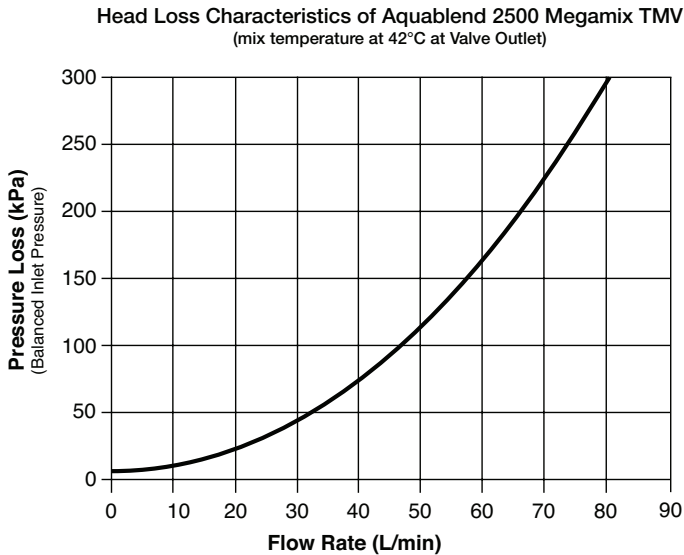
IMAGE 3 - Headloss Characteristics
