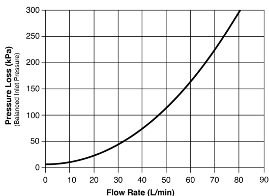
Head Loss Characteristics of Aquablend 2500 Megamix TMV (mix temperature at 42°C at Valve Outlet)
