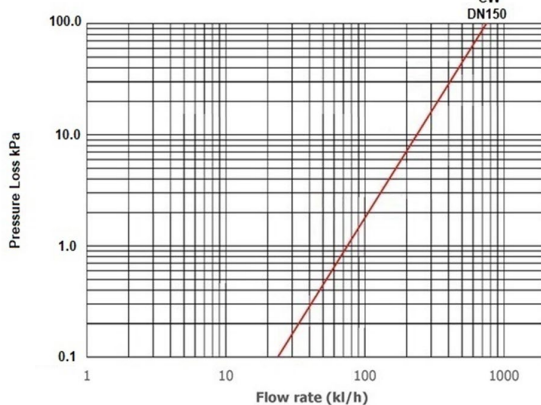
Pressure Loss Graph
