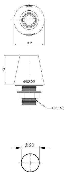
INSTALLATION DETAIL (BENCHTOP CUT OUT)
