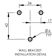
WALL BRACKET INSTALLATION DETAIL
