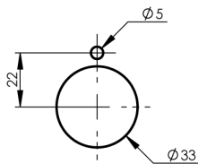
INSTALLATION DETAIL (MOUNTING SURFACE CUT OUT)
