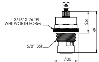
LEV380RTC
