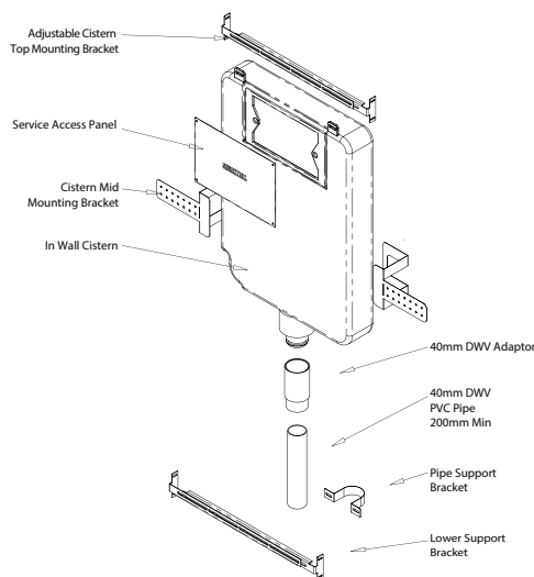
Fig 1: Exploded diagram
