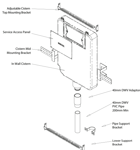
Fig 1: Exploded diagram
