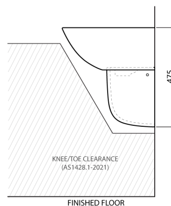
WB-BSNTYPB-E basin with WB-SHRD-E600 shroud
