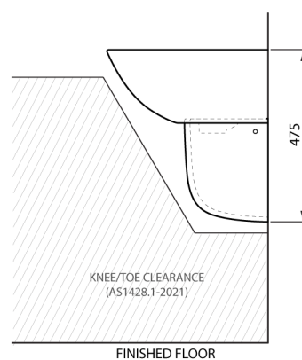
WB-BSNTYPB-E basin with WB-SHRD-E600 shroud
