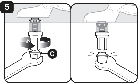
Tighten (C) until lower portions snap off.
