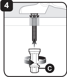
Finger tighten (C) to the under side of the bowl.
