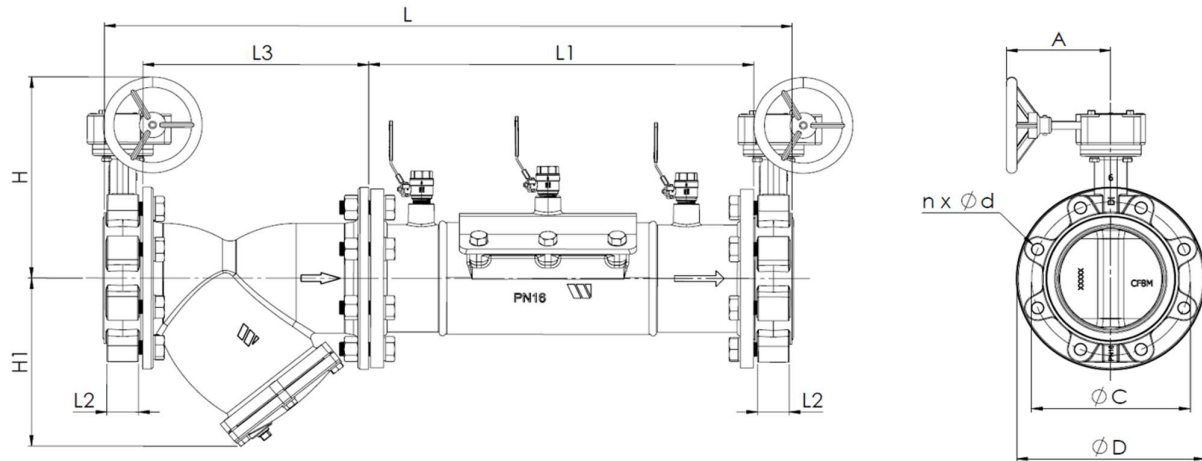
DCV Butterfly Valve with Gearbox
