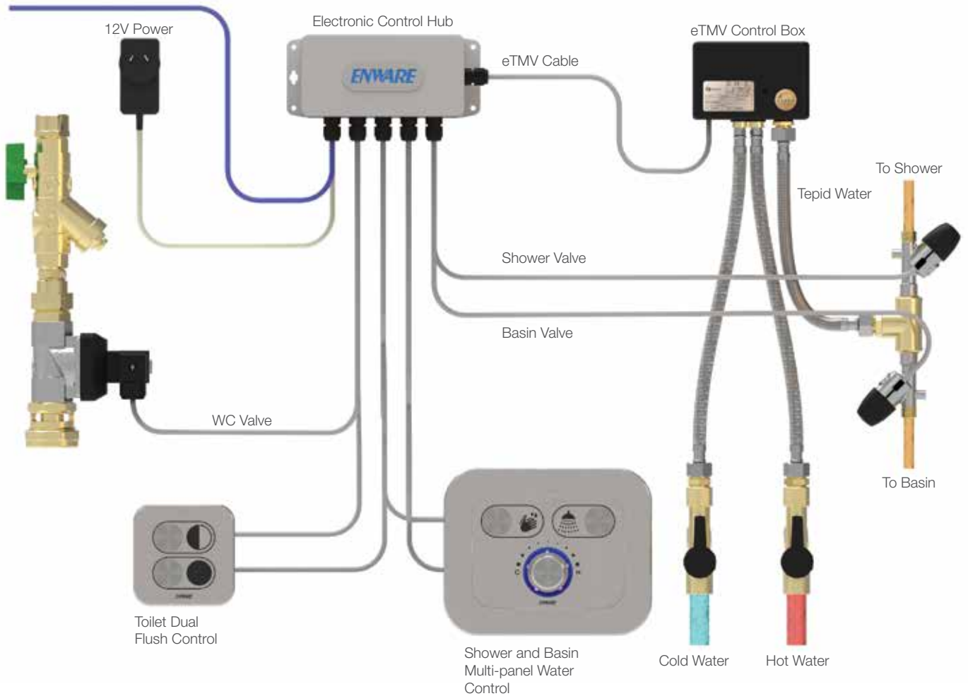
Smart Flow® LAN and Backbone Connection
